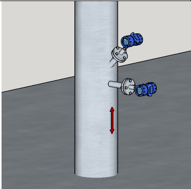
Mounted a vertical pipe with a diameter of 8 inches or larger. Mounted at 45° it can be mounted on smaller pipes. The flow can be downwards only if the pipe is completely full (No waterfall effect).
