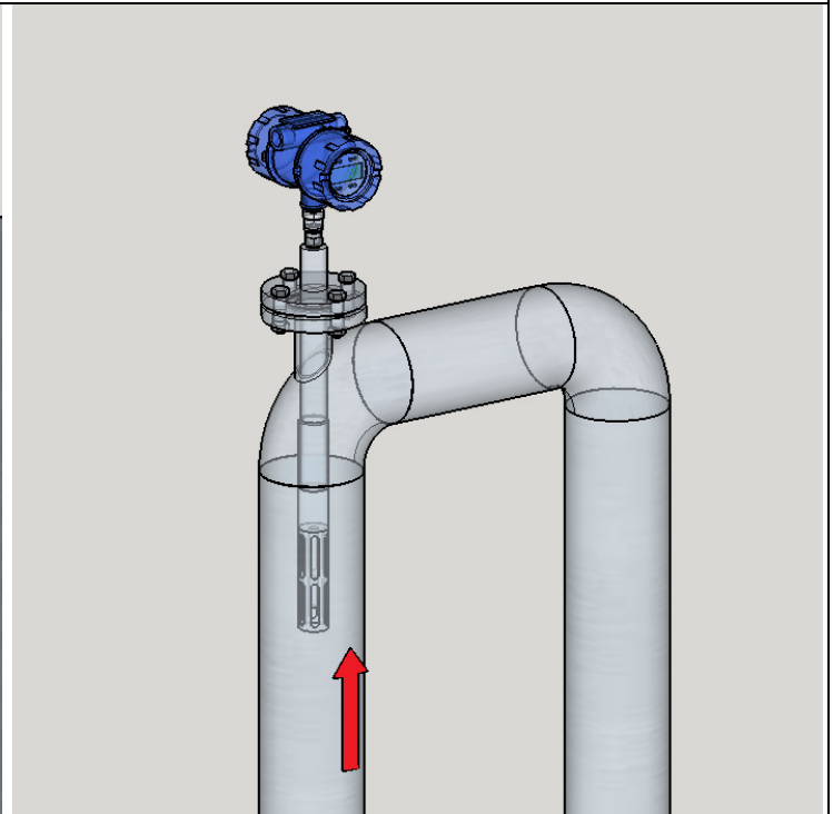
Mounted vertically on an elbow on pipes with diameter of 2 inches or larger. Notice that the cage has to be located deep into the vertical line to avoid the "Gas Trap" section at the top.
