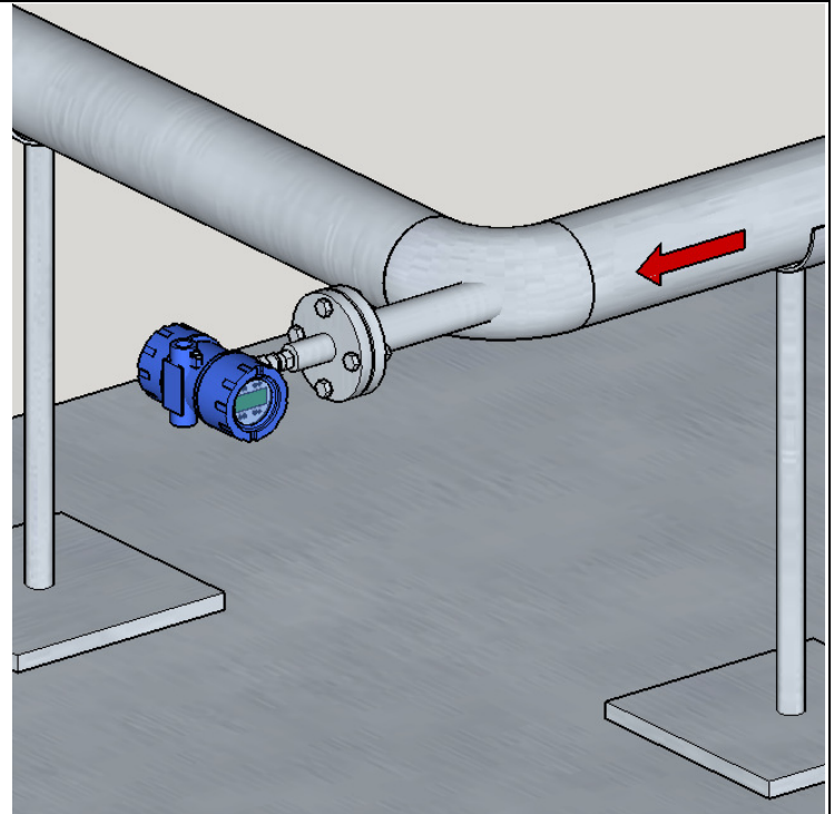
Mounted horizontally on an elbow on pipes with a diameter of 2 inches or larger
